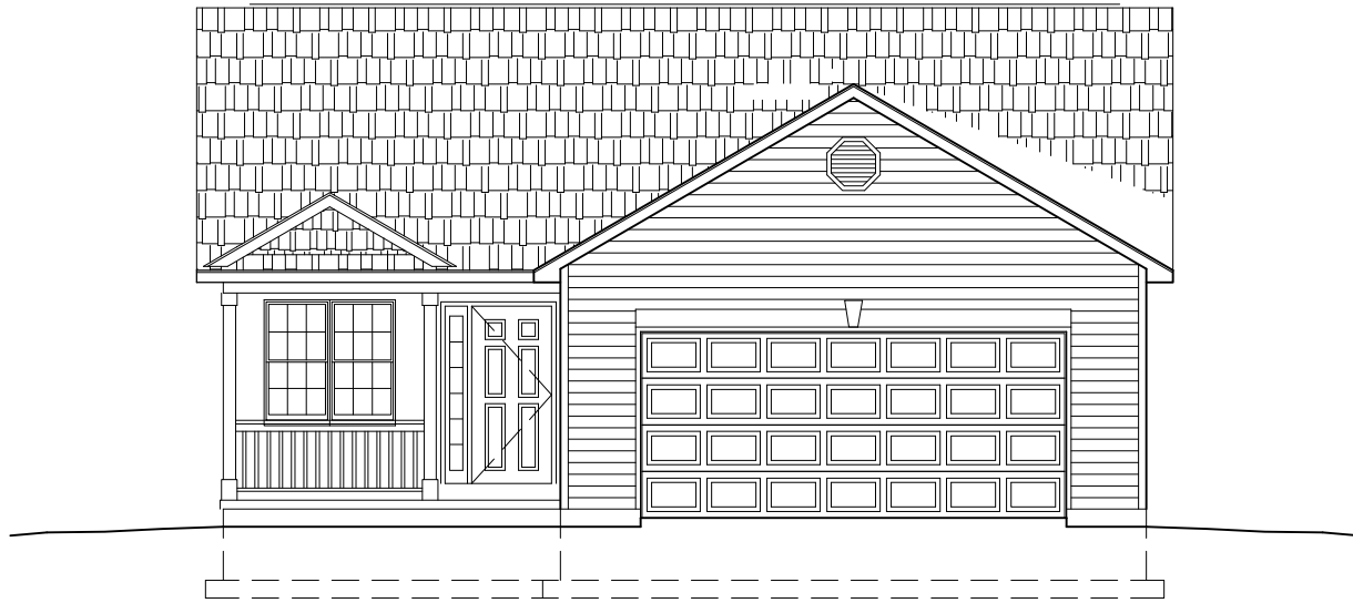
FRONT ELEVATION A-1
